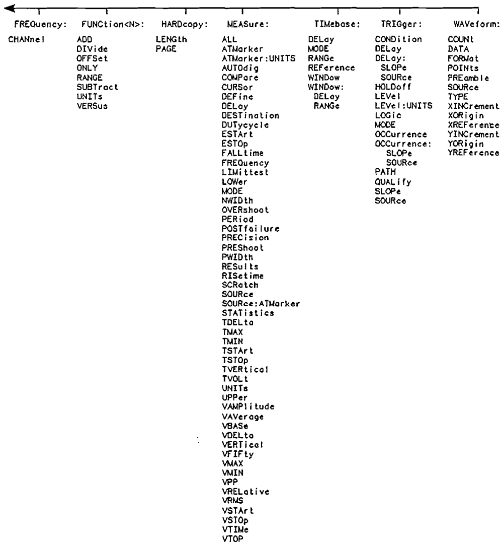
Figure 4-1. The HP 8990A Command Tree (continued)
