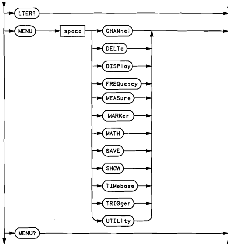
Figure 6-1. Root Level Commands Syntax Diagrams (continued)
