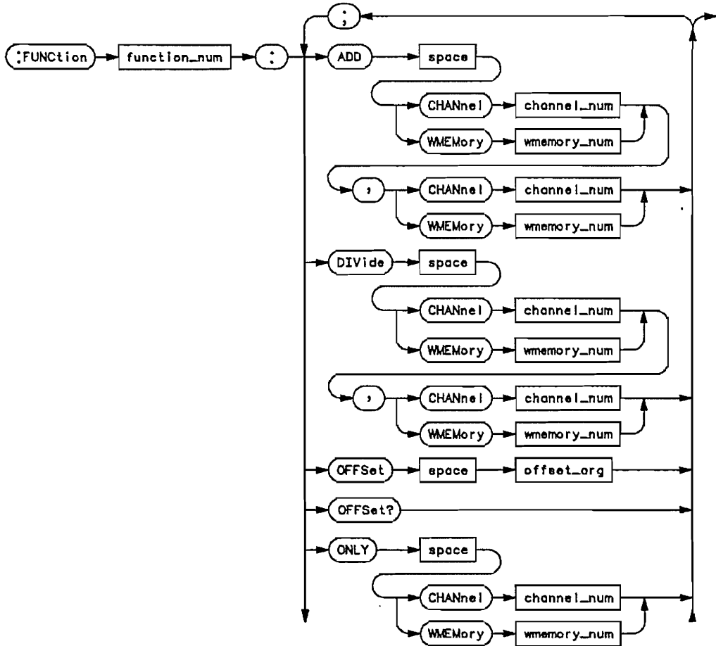
Figure 13-1. Function Subsystem Syntax Diagrams
