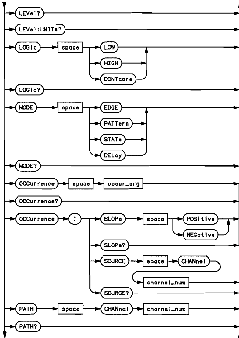
Figure 17-1. Trigger Subsystem Syntax Diagrams (continued)
