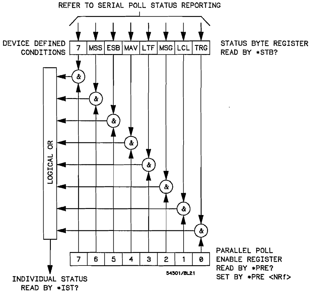
Figure 3-32. Parallel Poll Data Structure
