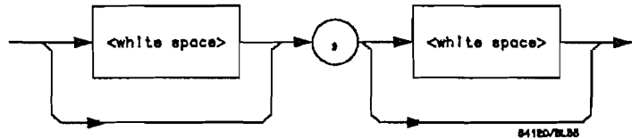
Figure 3-16. <program data separator>
