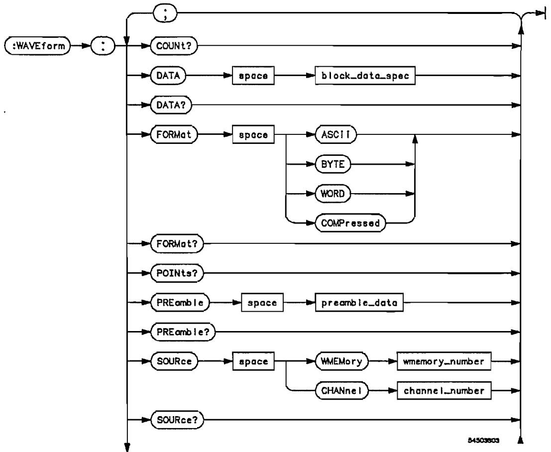
Figure 18-1. Waveform Subsystem Syntax Diagrams
