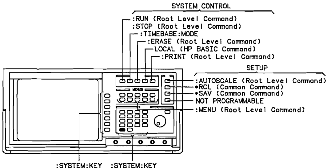
Figure 4-3. Front Panel Keys and Related HP-IB Commands
