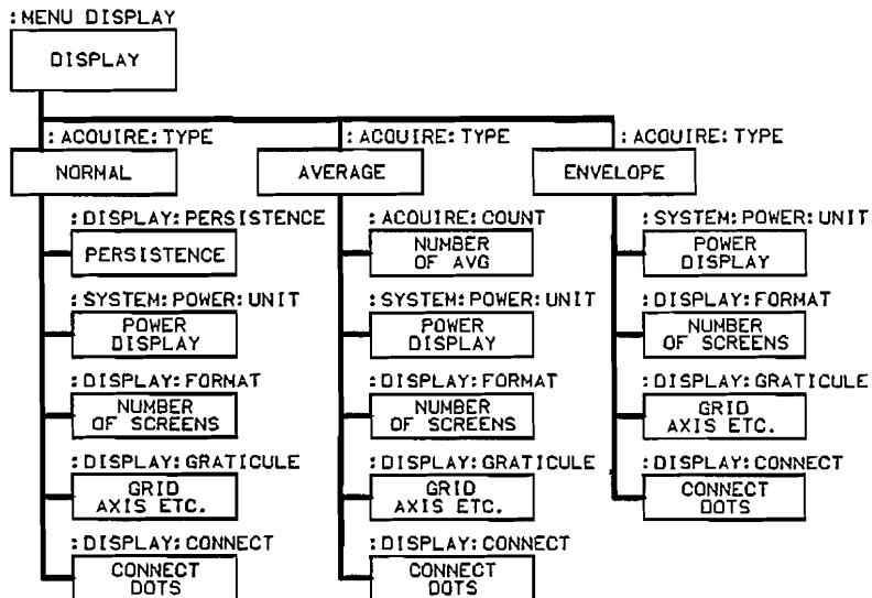
Figure 4-2. Front Panel Menus and Related HP-IB Commands (continued)
